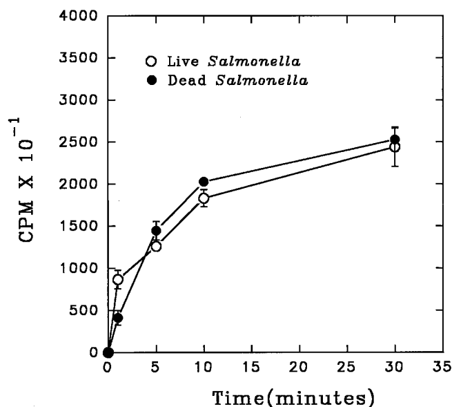
FIG. 1. Uptake of [ 35 S]methionine-labeled live or dead Salmonella by macrophages. Dead or live [ 35 S]methionine-labeled Salmonella ( 1 \times 10^7 ) were added to a 24-well plate containing 1 \times 10^6 J774E macrophages, and the infection was synchronized by low speed centrifugation at 4 °C as described under "Experimental Procedures." After incubation for the indicated time periods at 37 °C, cells were washed extensively to remove unbound bacteria and solubilized with 1% Triton X-100. An aliquot was used to determine radioactivity in a \beta -counter, and the results were expressed as the means \pm S.D. of three determinations. Specific activity of live and dead Salmonella were 0.8 cpm/bacteria.
